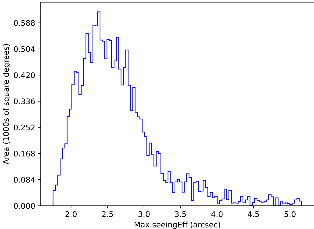
internal_u_expt60_nscale1.2v3.4_10yrs WFD i band: Max seeingEff
