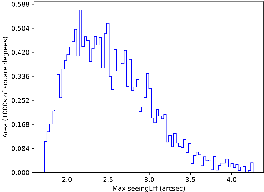
internal_u_expt60_nscale1.2v3.4_10yrs WFD g band: Max seeingEff
