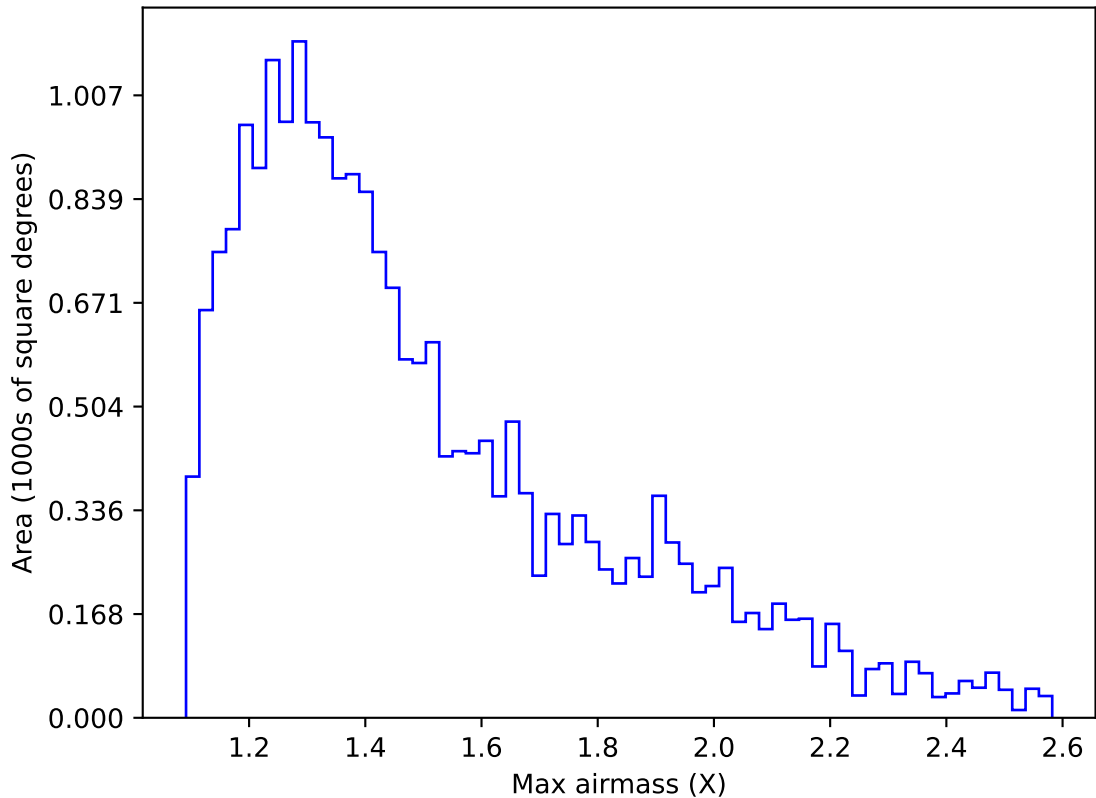
internal_u_expt60_nscale1.2v3.4_10yrs Yr 1 u band: Max airmass
