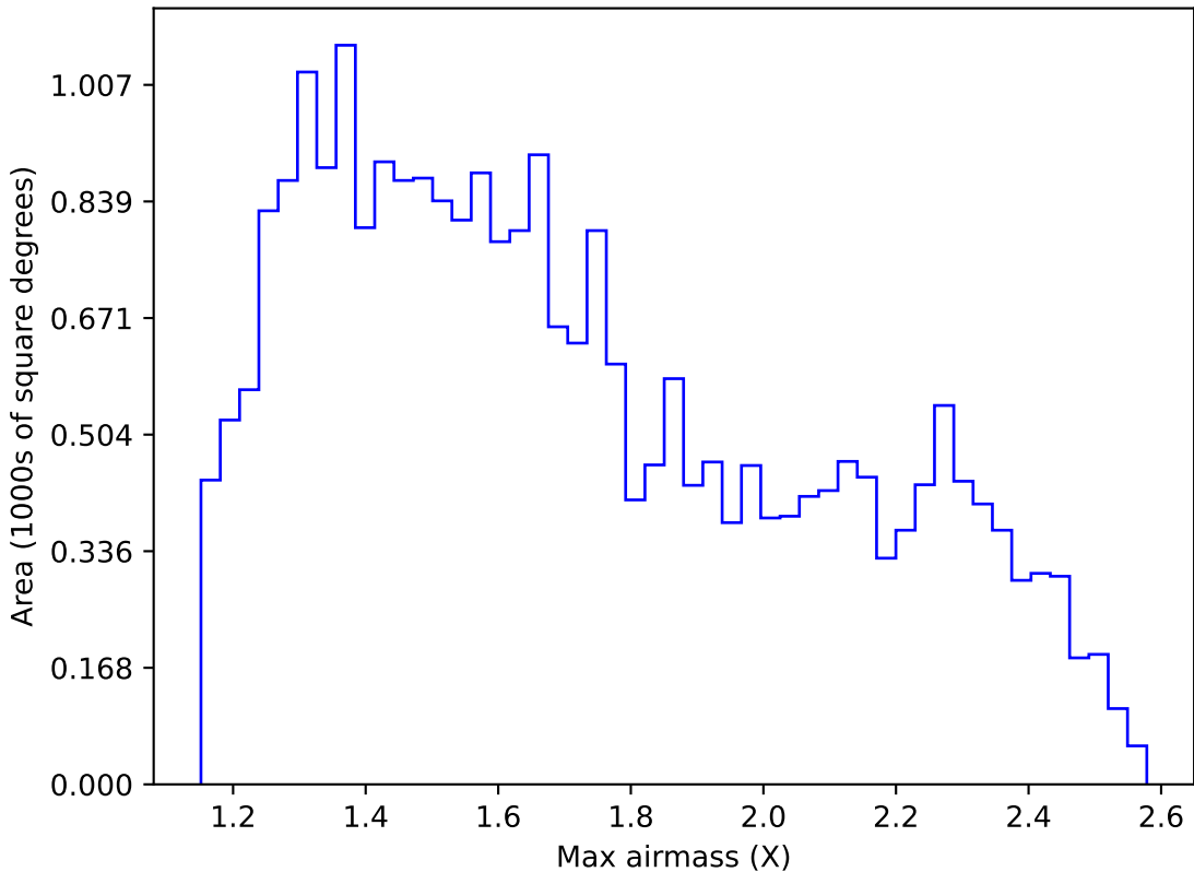
internal_u_expt60_nscale1.2v3.4_10yrs Yr 1 r band: Max airmass
