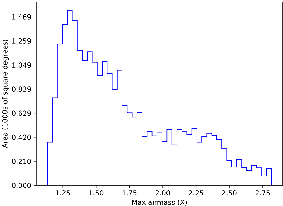
internal_u_expt60_nscale1.2v3.4_10yrs Yr 1 i band: Max airmass
