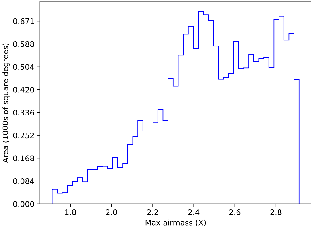
internal_u_expt60_nscale1.2v3.4_10yrs WFD z band: Max airmass
