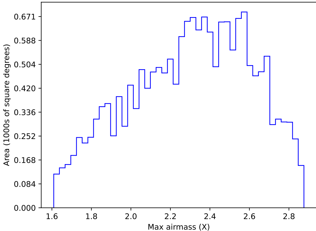
internal_u_expt60_nscale1.2v3.4_10yrs WFD y band: Max airmass
