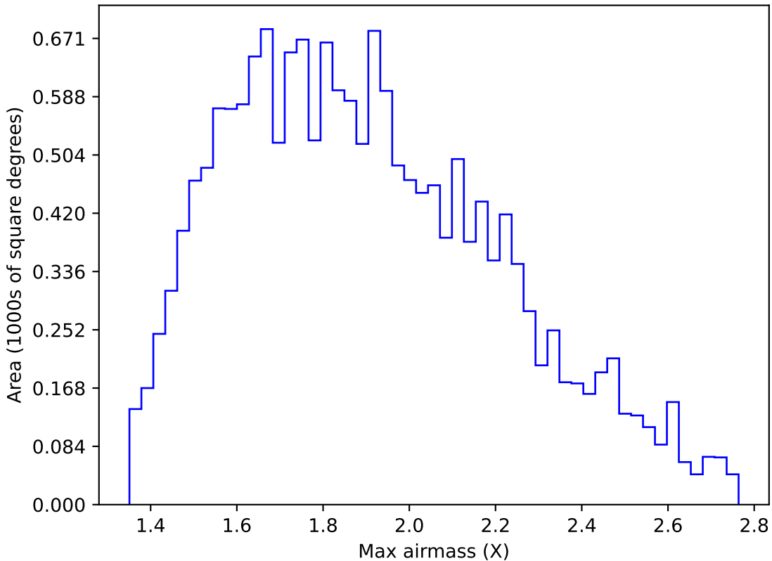
internal_u_expt60_nscale1.2v3.4_10yrs WFD u band: Max airmass
