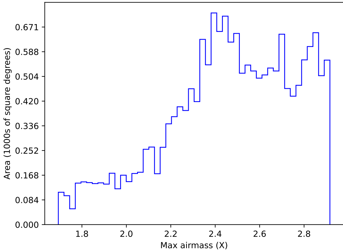
internal_u_expt60_nscale1.2v3.4_10yrs WFD i band: Max airmass
