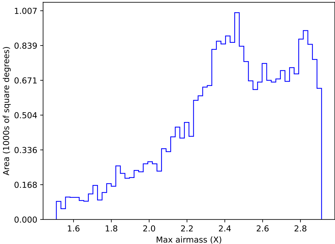
internal_u_expt60_nscale1.2v3.4_10yrs All sky z band: Max airmass
