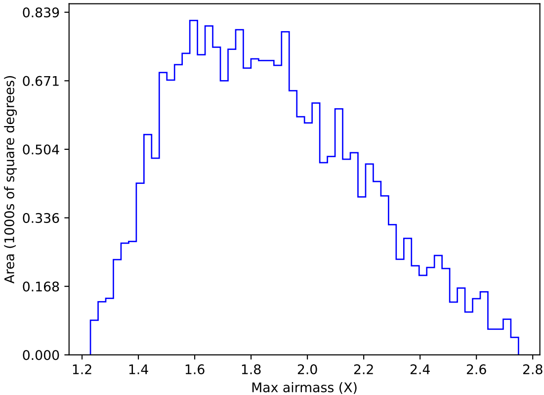
internal_u_expt60_nscale1.2v3.4_10yrs All sky u band: Max airmass
