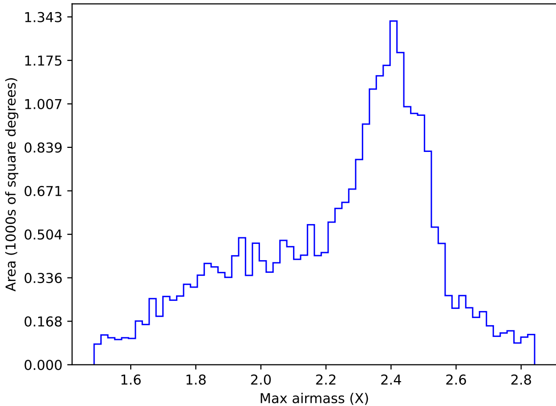
internal_u_expt60_nscale1.2v3.4_10yrs All sky r band: Max airmass
