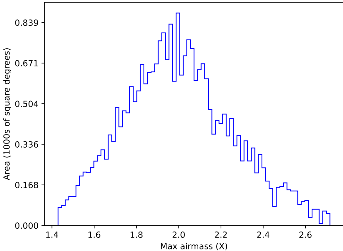
internal_u_expt60_nscale1.2v3.4_10yrs All sky g band: Max airmass
