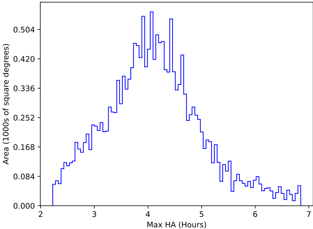
internal_u_expt60_nscale1.2v3.4_10yrs WFD u band: Max HA
