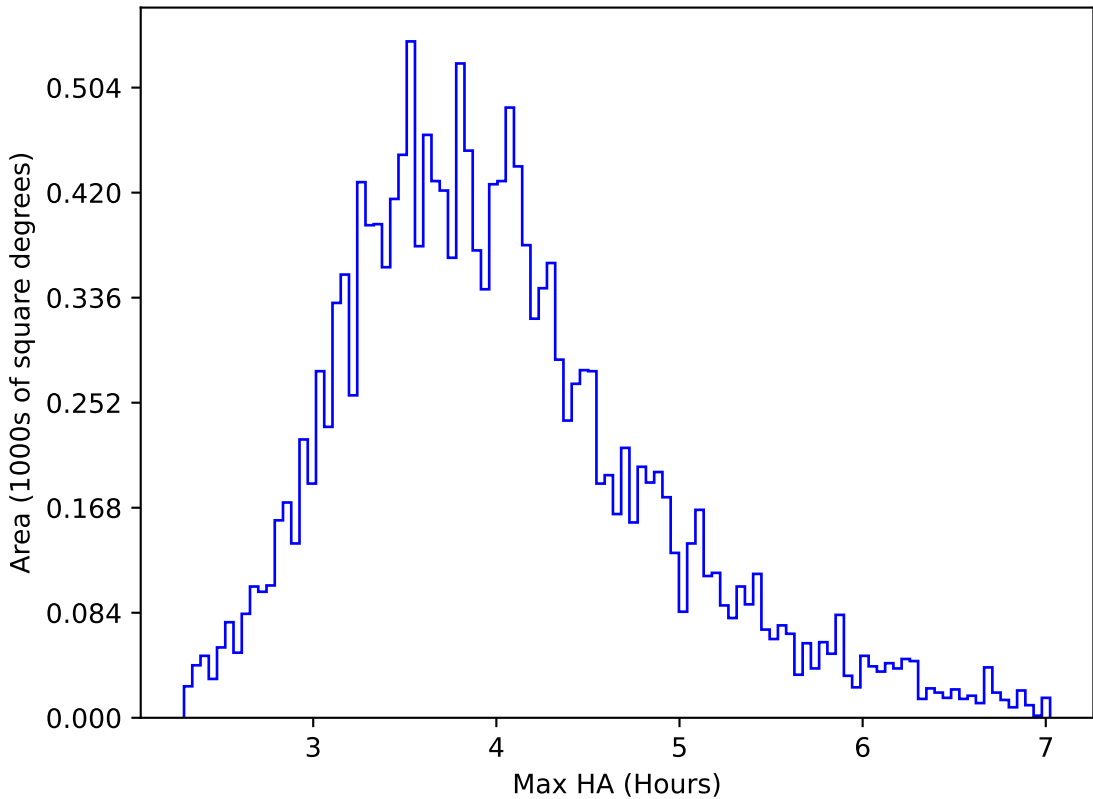
internal_u_expt60_nscale1.2v3.4_10yrs WFD g band: Max HA
