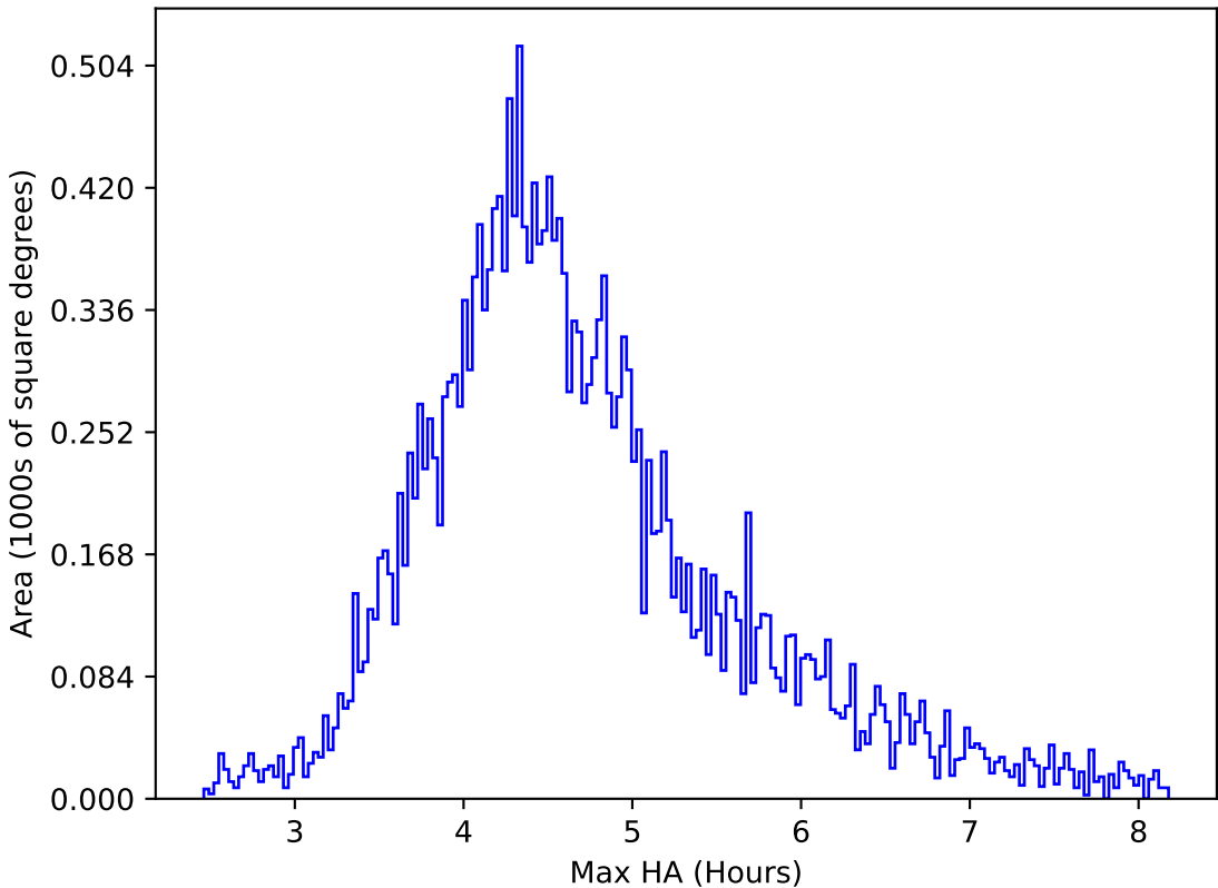
internal_u_expt60_nscale1.2v3.4_10yrs All sky y band: Max HA
