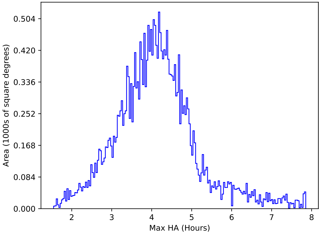
internal_u_expt60_nscale1.2v3.4_10yrs All sky r band: Max HA
