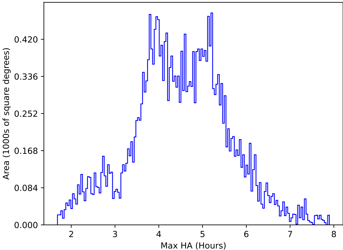
internal_u_expt60_nscale1.2v3.4_10yrs All sky i band: Max HA
