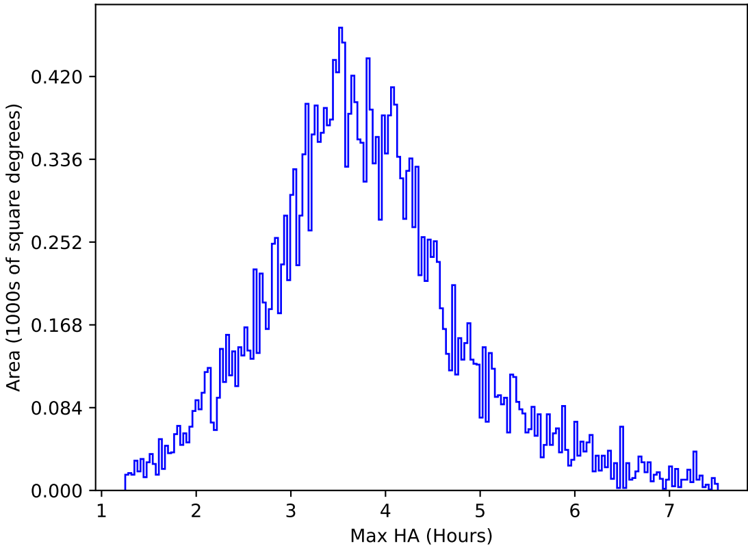
internal_u_expt60_nscale1.2v3.4_10yrs All sky g band: Max HA
