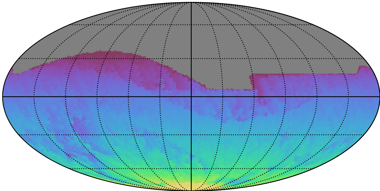
internal_u_expt60_nscale1.2v3.4_10yrs All sky all bands: Max HA
