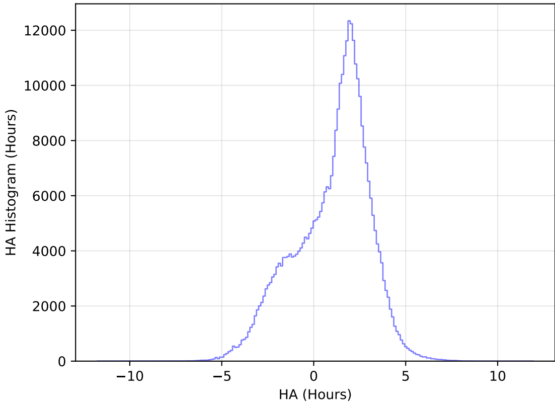
internal_u_expt60_nscale1.2v3.4_10yrs WFD y band: HA Histogram
