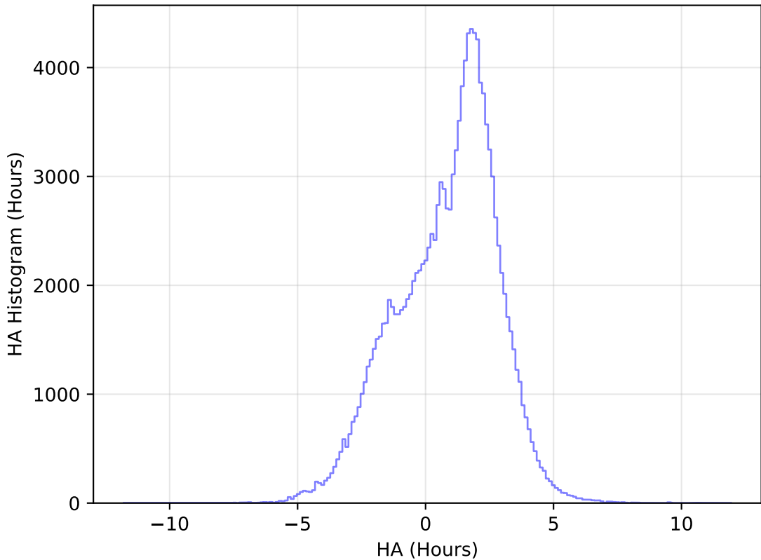
internal_u_expt60_nscale1.2v3.4_10yrs WFD u band: HA Histogram
