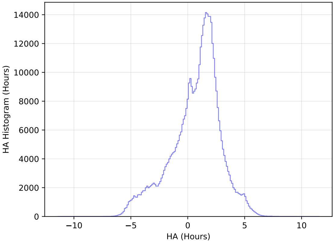
internal_u_expt60_nscale1.2v3.4_10yrs WFD i band: HA Histogram
