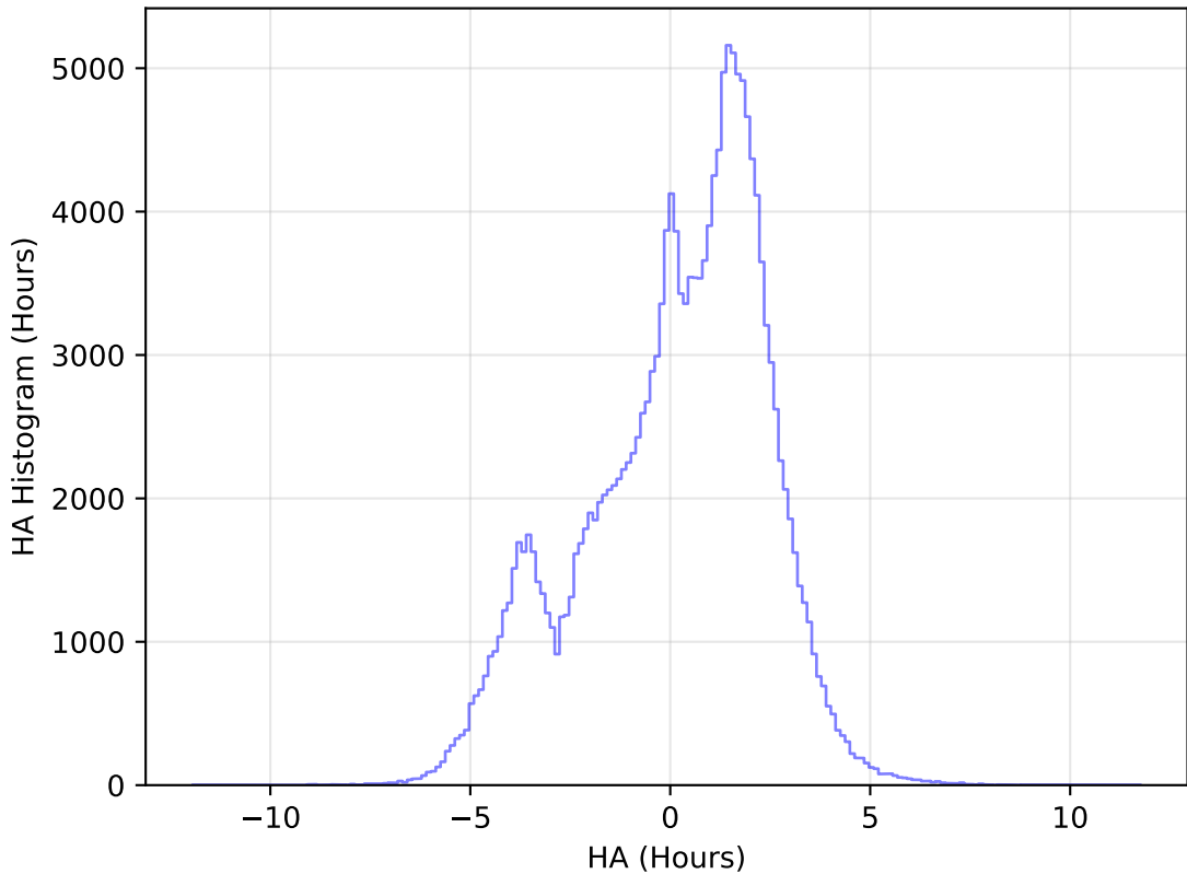
internal_u_expt60_nscale1.2v3.4_10yrs WFD g band: HA Histogram
