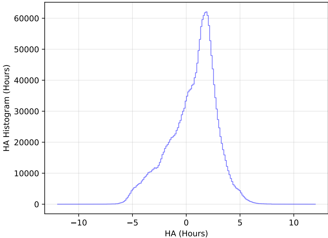
internal_u_expt60_nscale1.2v3.4_10yrs WFD all bands: HA Histogram
