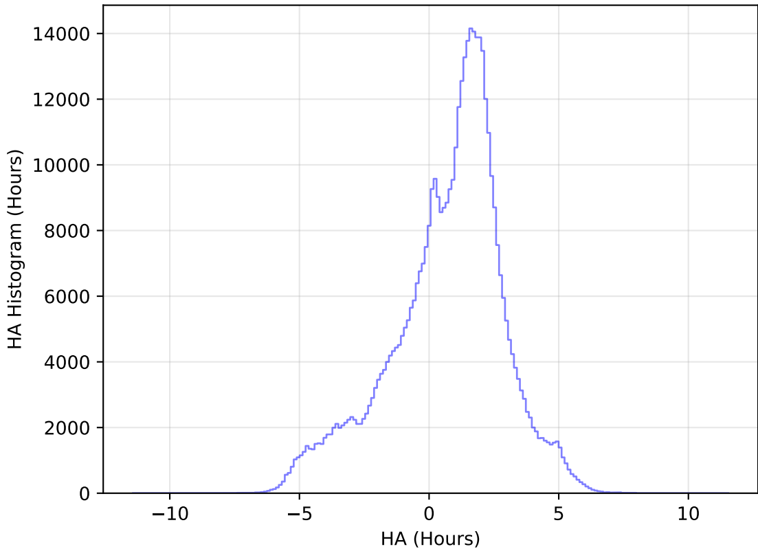
internal_u_expt60_nscale1.2v3.4_10yrs All sky i band: HA Histogram
