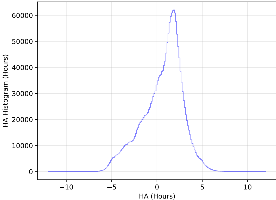
internal_u_expt60_nscale1.2v3.4_10yrs All sky all bands: HA Histogram
