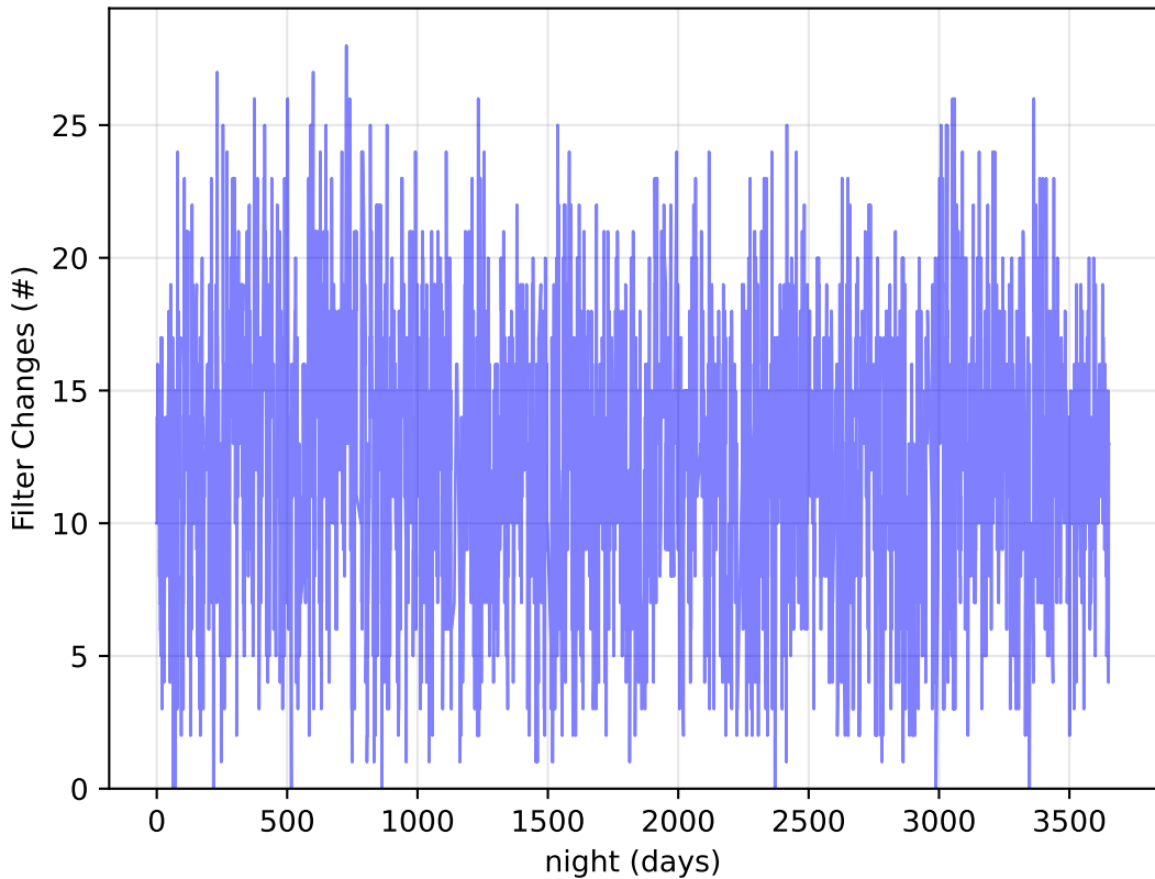
internal_u_expt60_nscale1.2v3.4_10yrs Per Night: Filter Changes
