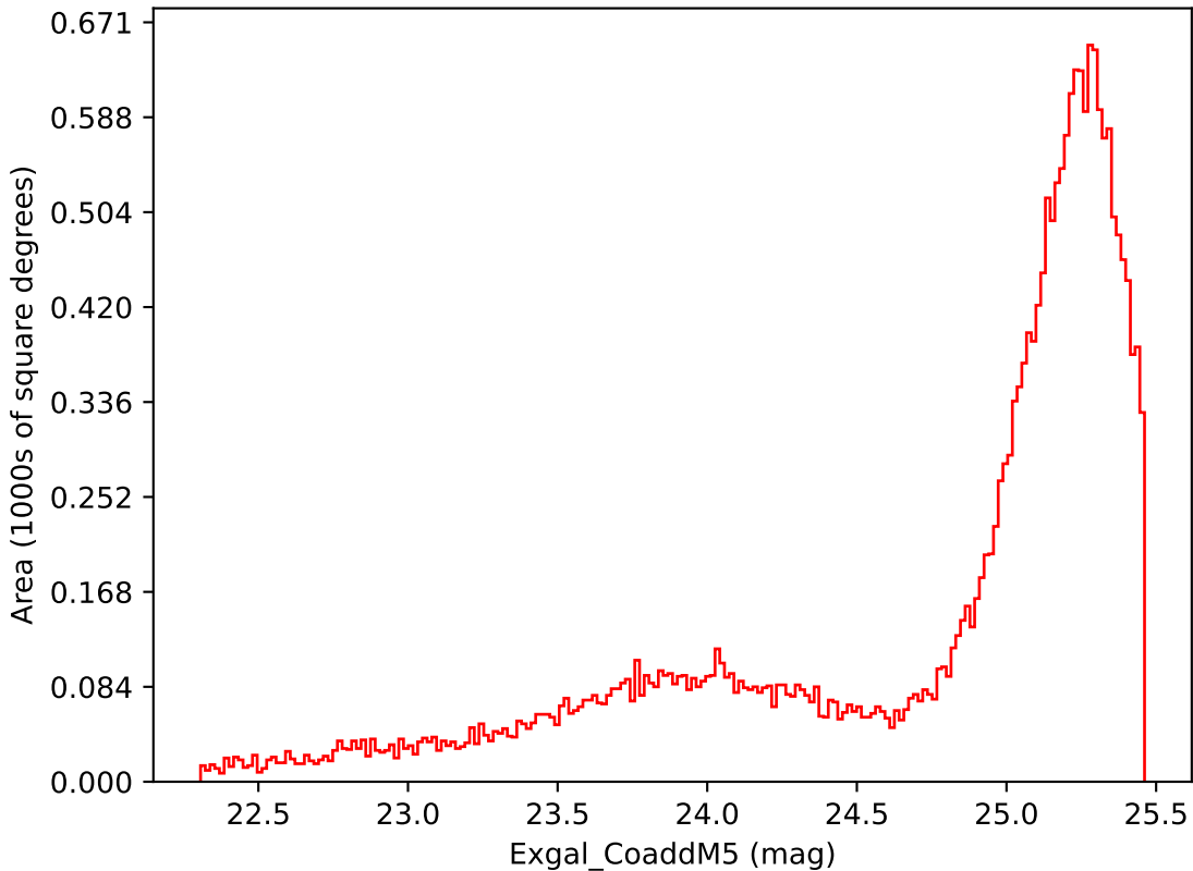
internal_u_expt60_nscale1.2v3.4_10yrs Yr 1 i band: Exgal_CoaddM5
