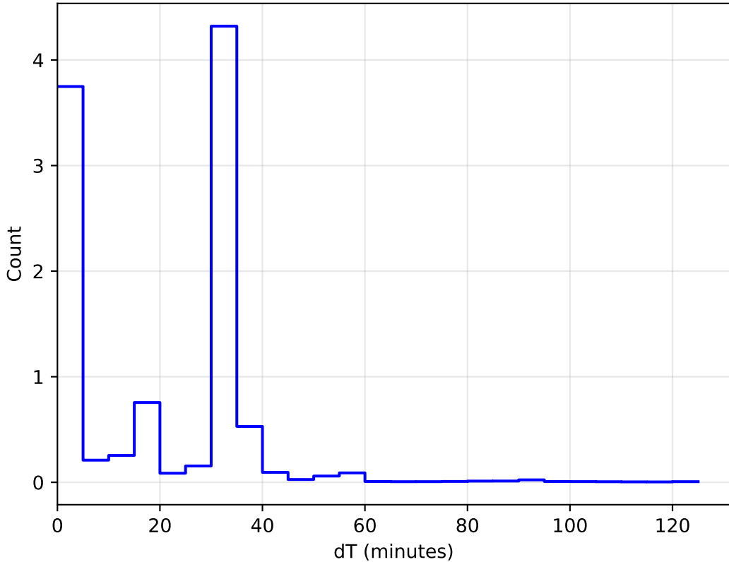
internal_u_expt60_nscale1.2v3.4_10yrs WFD: DeltaT Histogram
