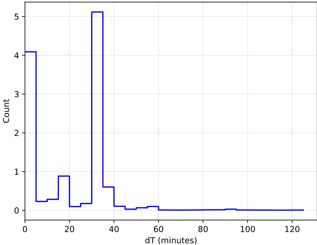
internal_u_expt60_nscale1.2v3.4_10yrs All sky: DeltaT Histogram
