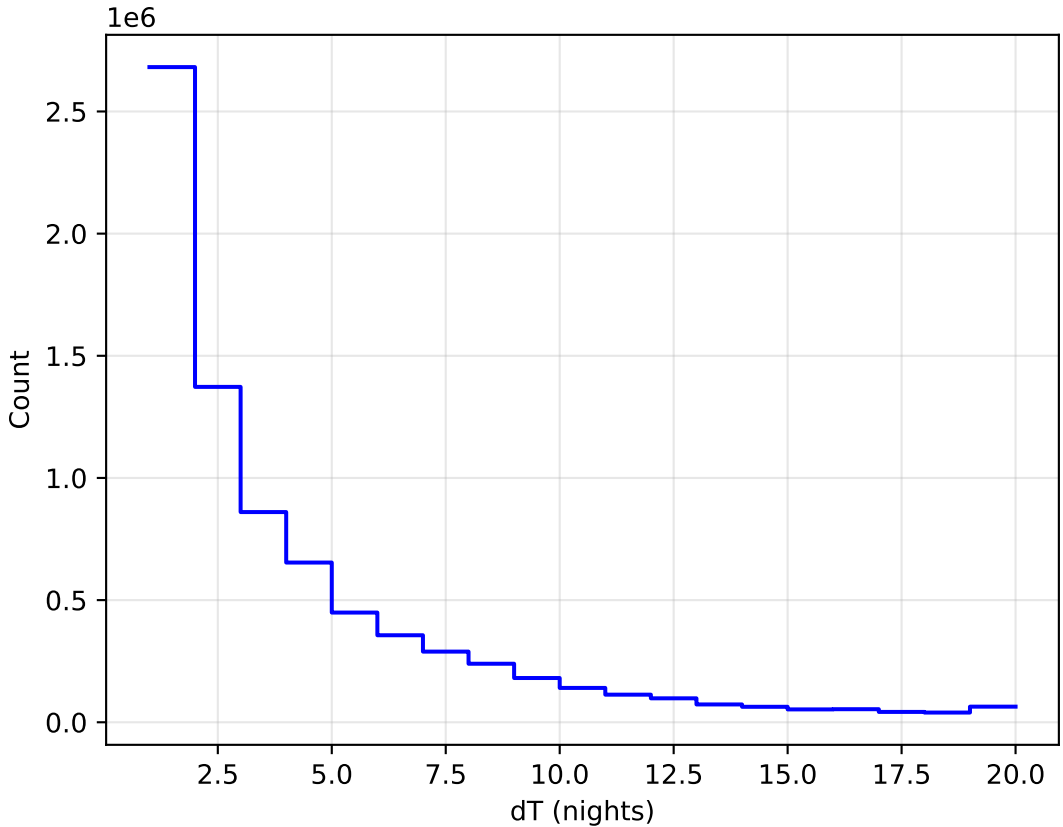
internal_u_expt60_nscale1.2v3.4_10yrs WFD all bands: DeltaNight Histogram
