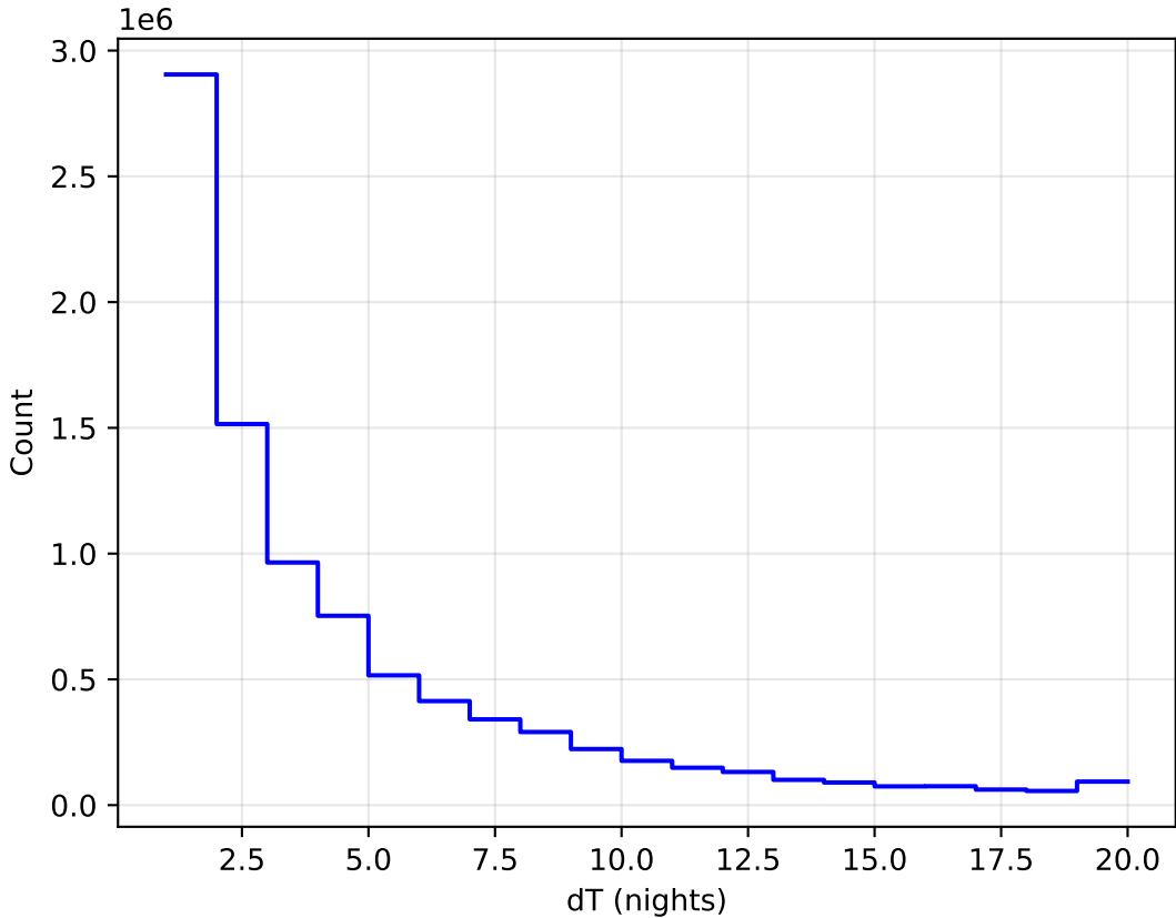
internal_u_expt60_nscale1.2v3.4_10yrs All sky all bands: DeltaNight Histogram
