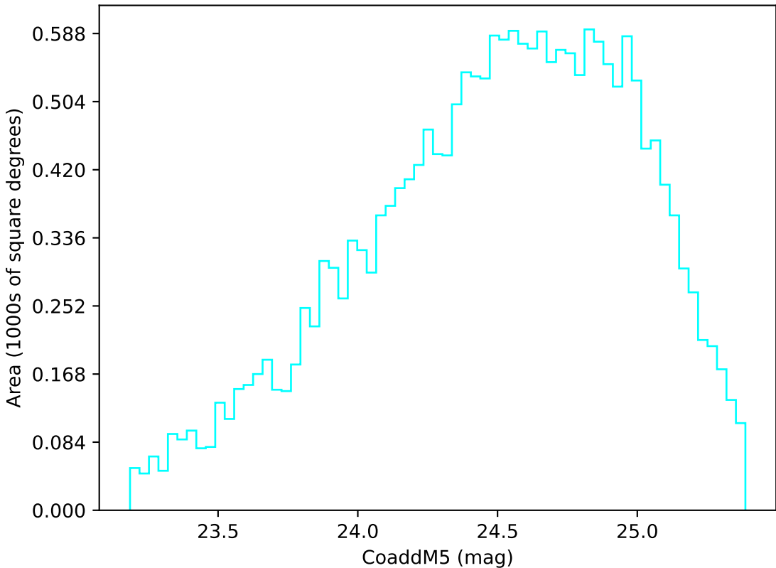
internal_u_expt60_nscale1.2v3.4_10yrs Yr 3-4 u band: CoaddM5
