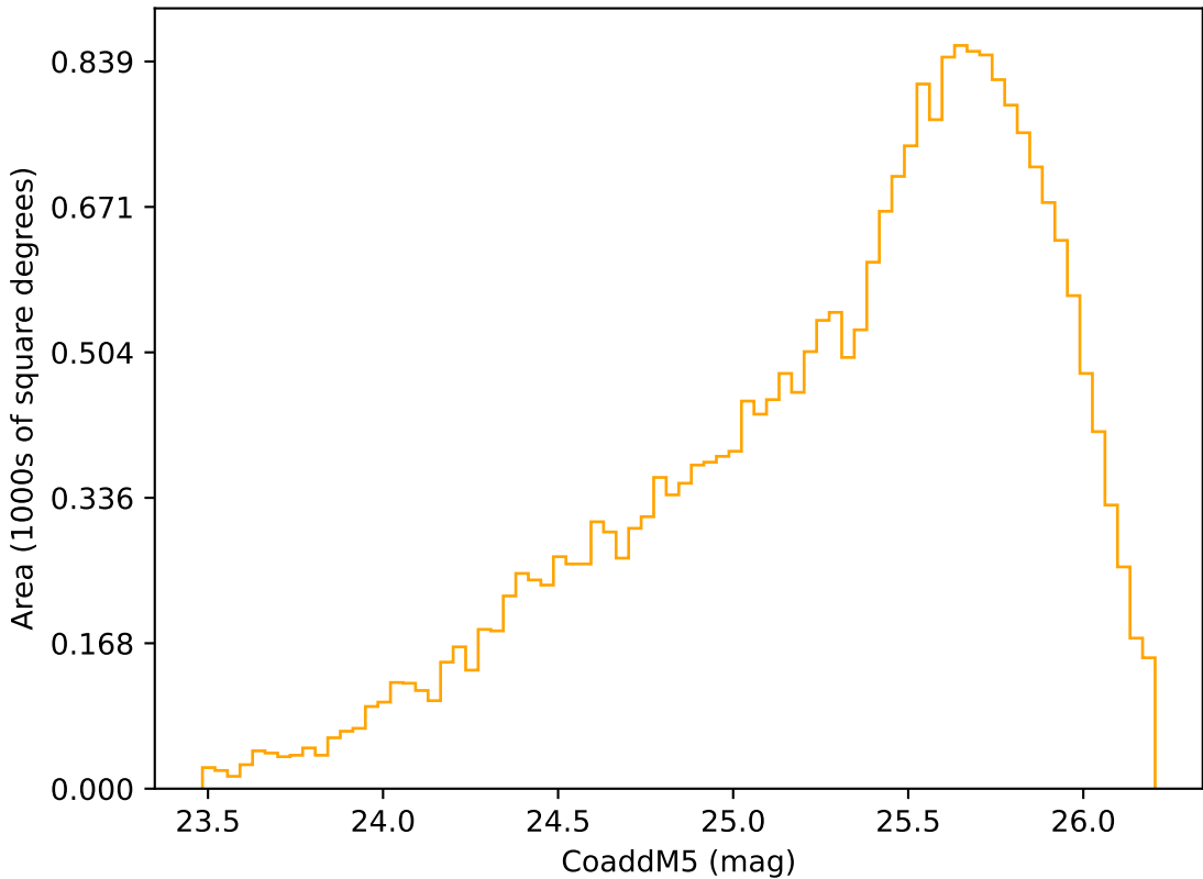
internal_u_expt60_nscale1.2v3.4_10yrs Yr 3-4 r band: CoaddM5
