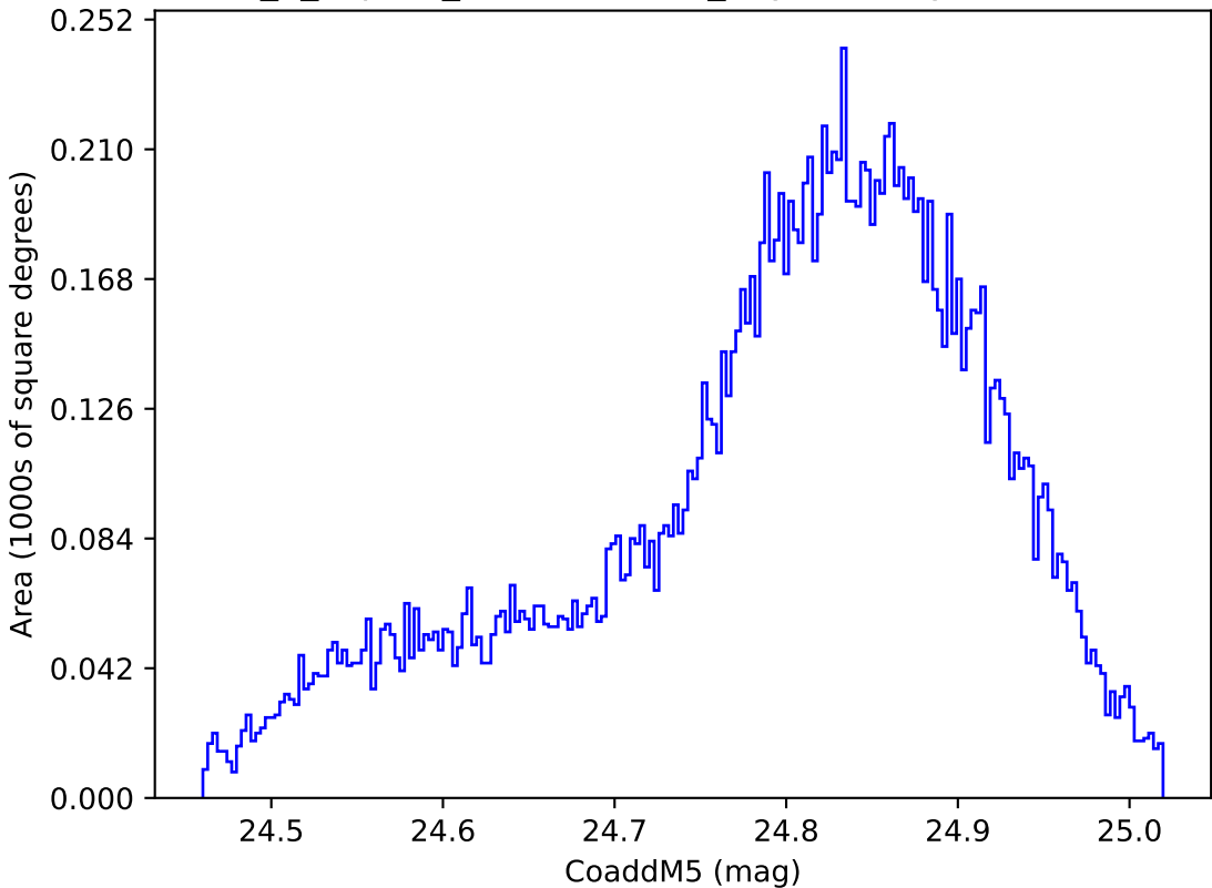
internal_u_expt60_nscale1.2v3.4_10yrs WFD y band: CoaddM5
