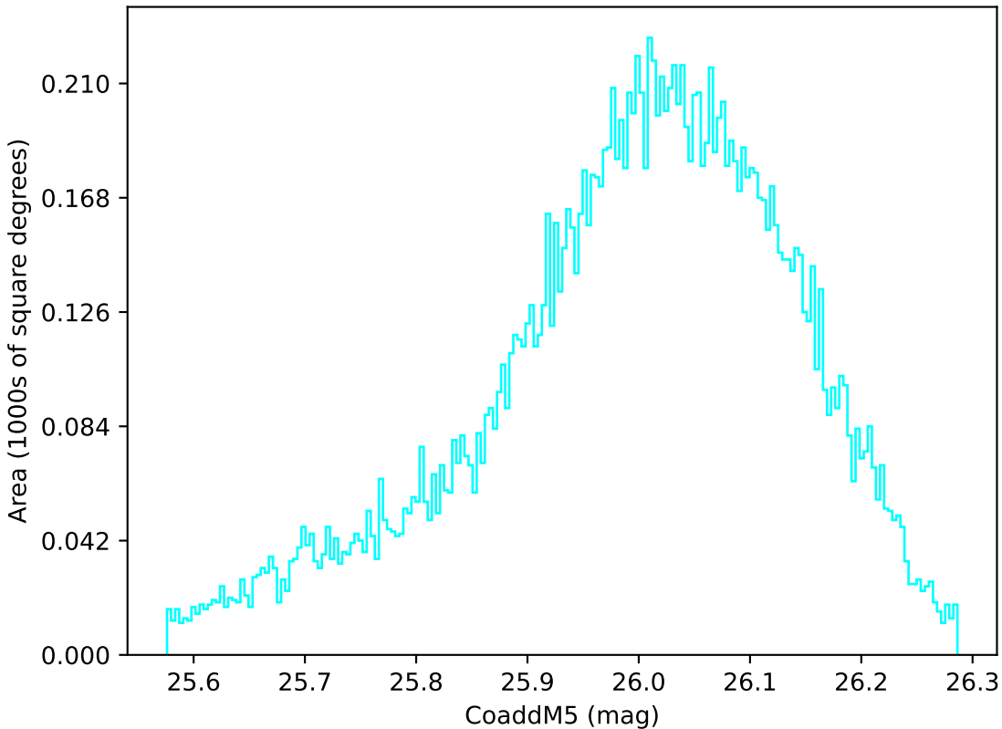
internal_u_expt60_nscale1.2v3.4_10yrs WFD u band: CoaddM5
