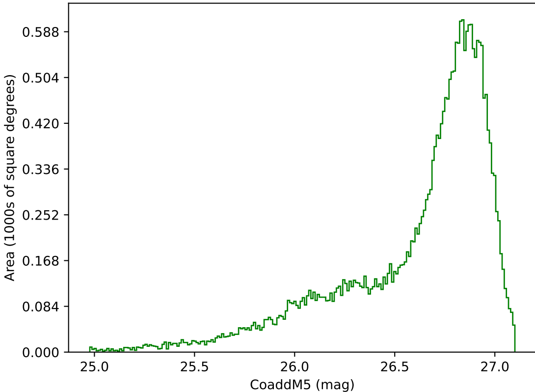
internal_u_expt60_nscale1.2v3.4_10yrs All sky g band: CoaddM5
