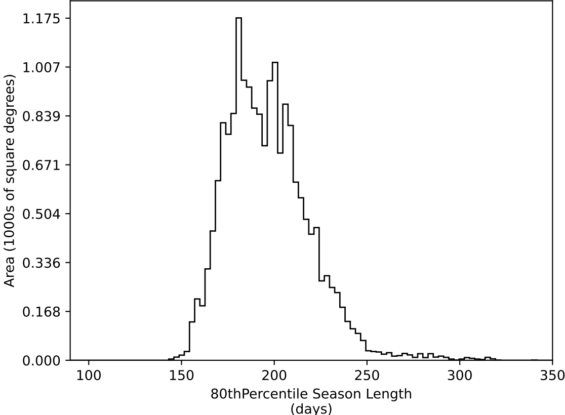
internal_u_expt60_nscale1.2v3.4_10yrs WFD all bands: 80thPercentile Season Length
