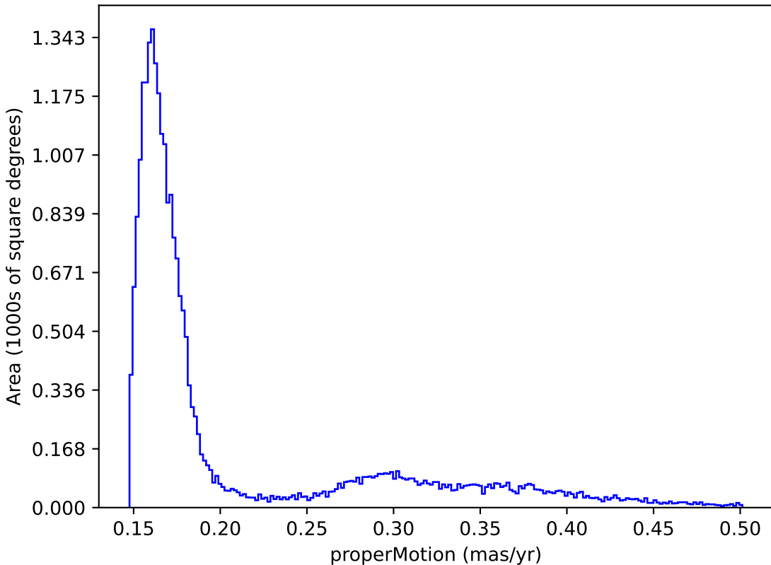
internal_u_expt60_nscale1.2v3.4_10yrs : properMotion
