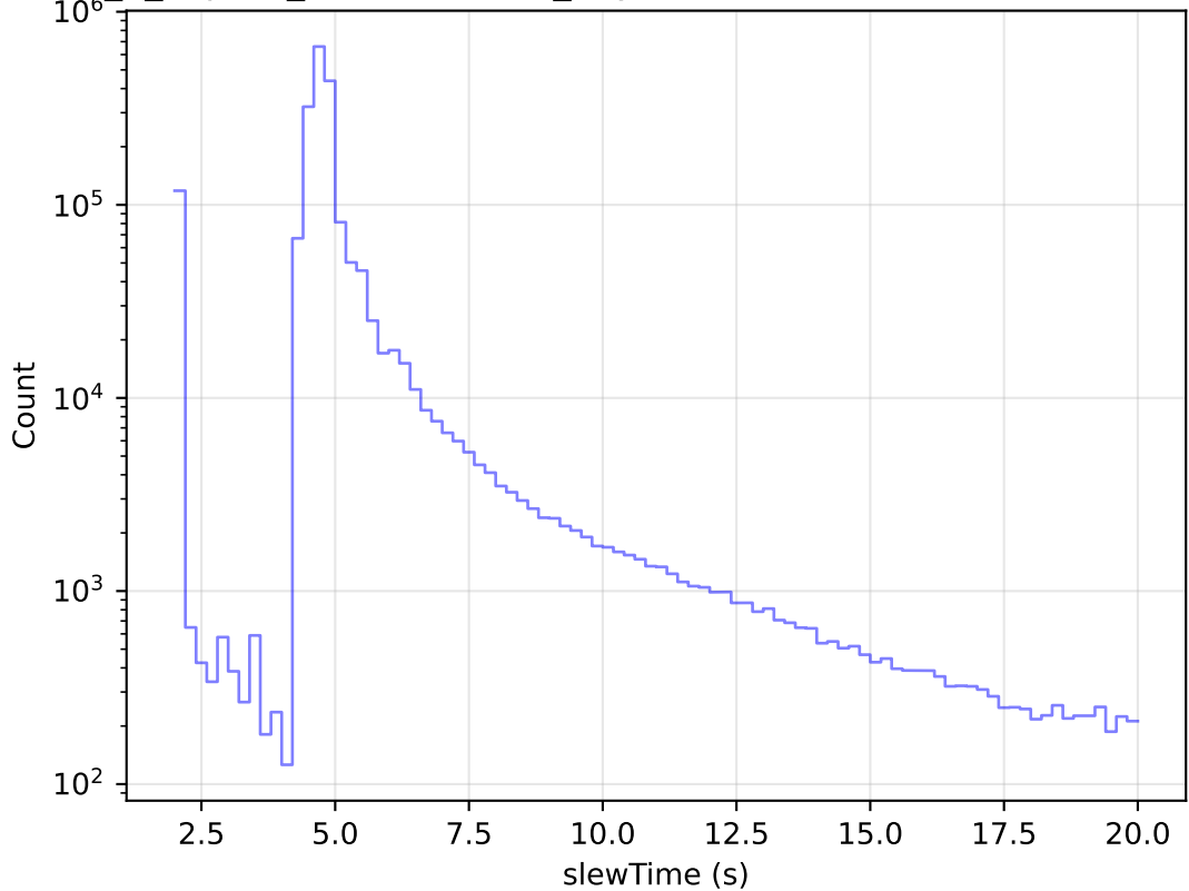
internal_u_expt60_nscale1.2v3.4_10yrs All visits: Zoom Slew Time Histogram
