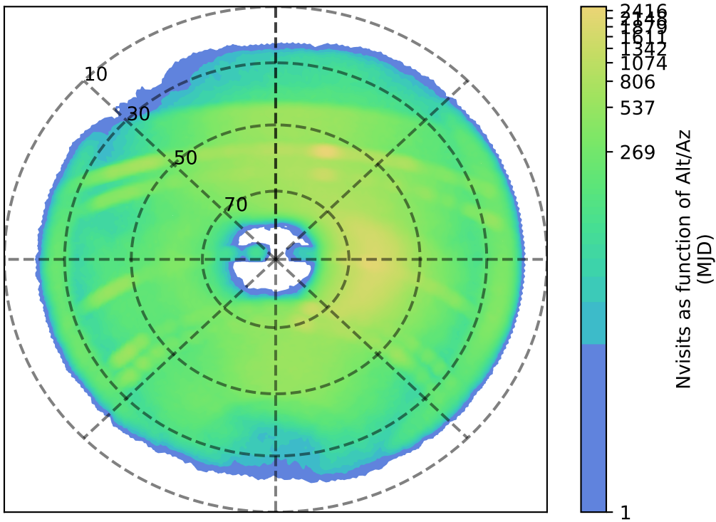
internal_u_expt60_nscale1.2v3.4_10yrs z: Nvisits as function of Alt/Az
