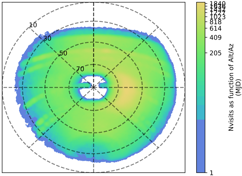
internal_u_expt60_nscale1.2v3.4_10yrs y: Nvisits as function of Alt/Az
