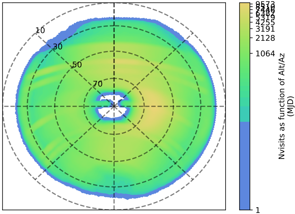
internal_u_expt60_nscale1.2v3.4_10yrs : Nvisits as function of Alt/Az
