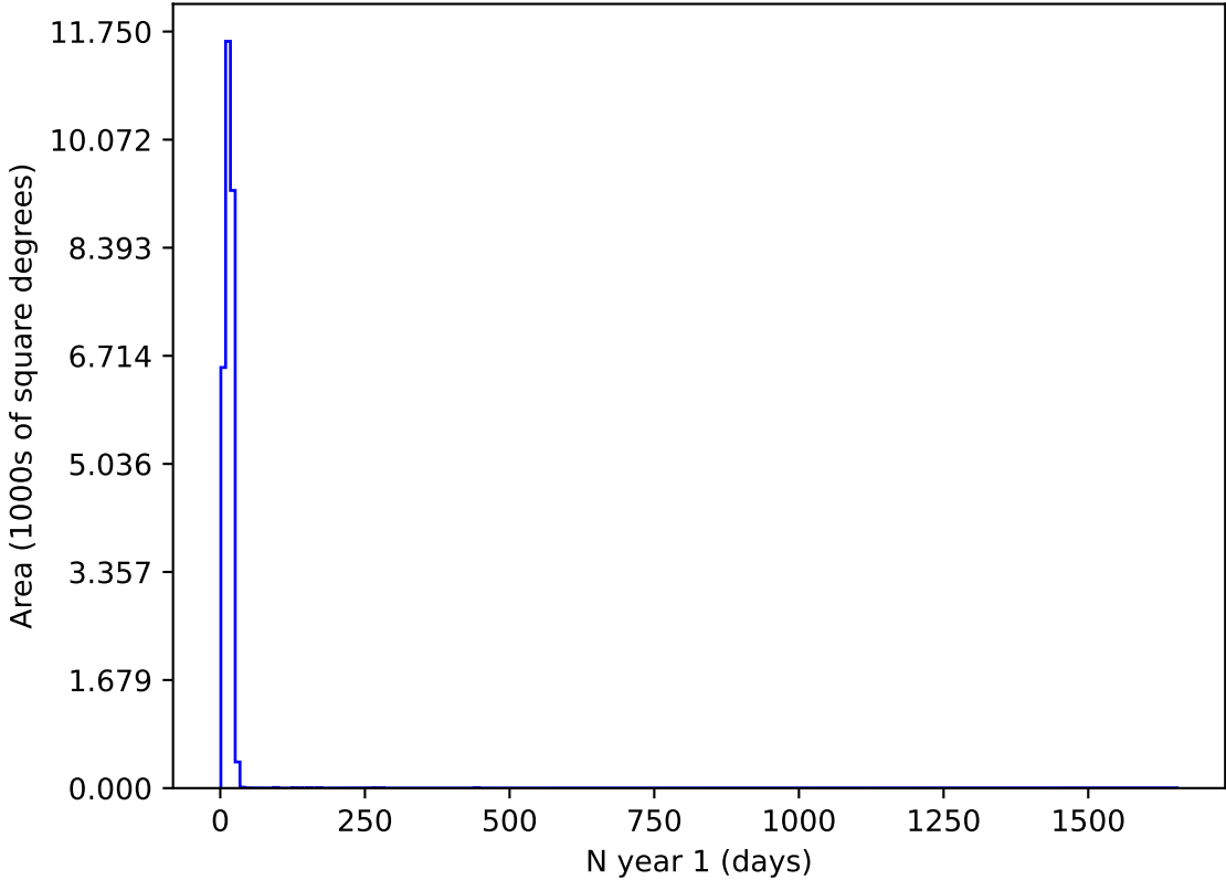
internal_u_expt60_nscale1.2v3.4_10yrs r and night < 365: N year 1
