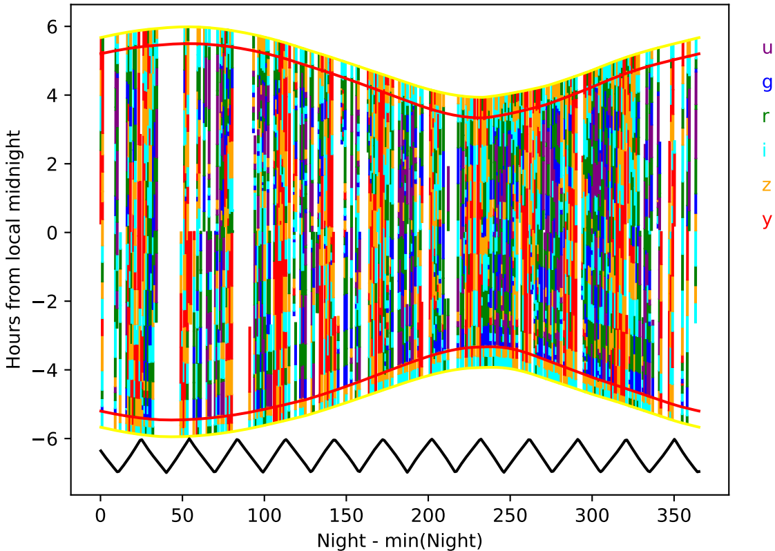
internal_u_expt60_nscale1.2v3.4_10yrs year 4-5: Hourglass
