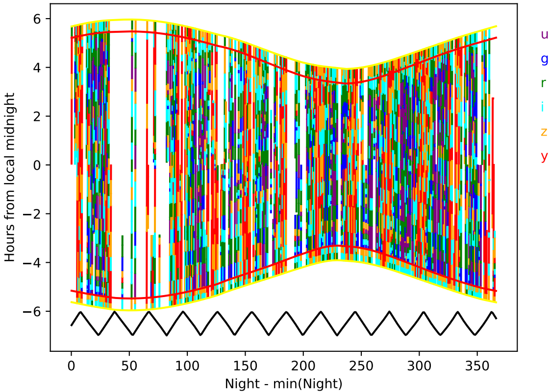
internal_u_expt60_nscale1.2v3.4_10yrs year 3-4: Hourglass
