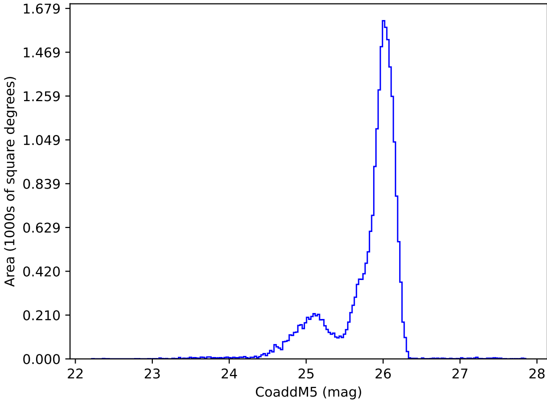
internal_u_expt60_nscale1.2v3.4_10yrs u: CoaddM5
