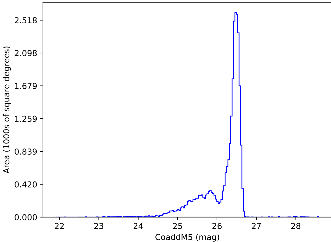
internal_u_expt60_nscale1.2v3.4_10yrs i: CoaddM5
