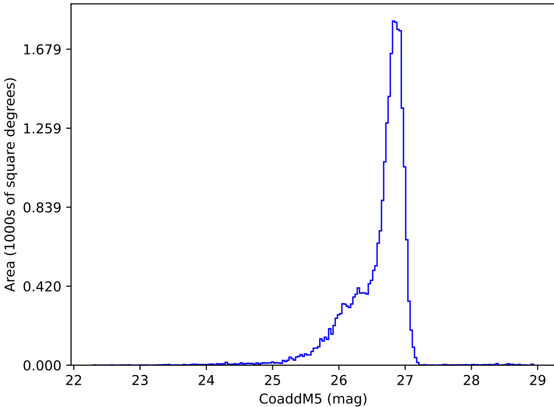
internal_u_expt60_nscale1.2v3.4_10yrs g: CoaddM5
